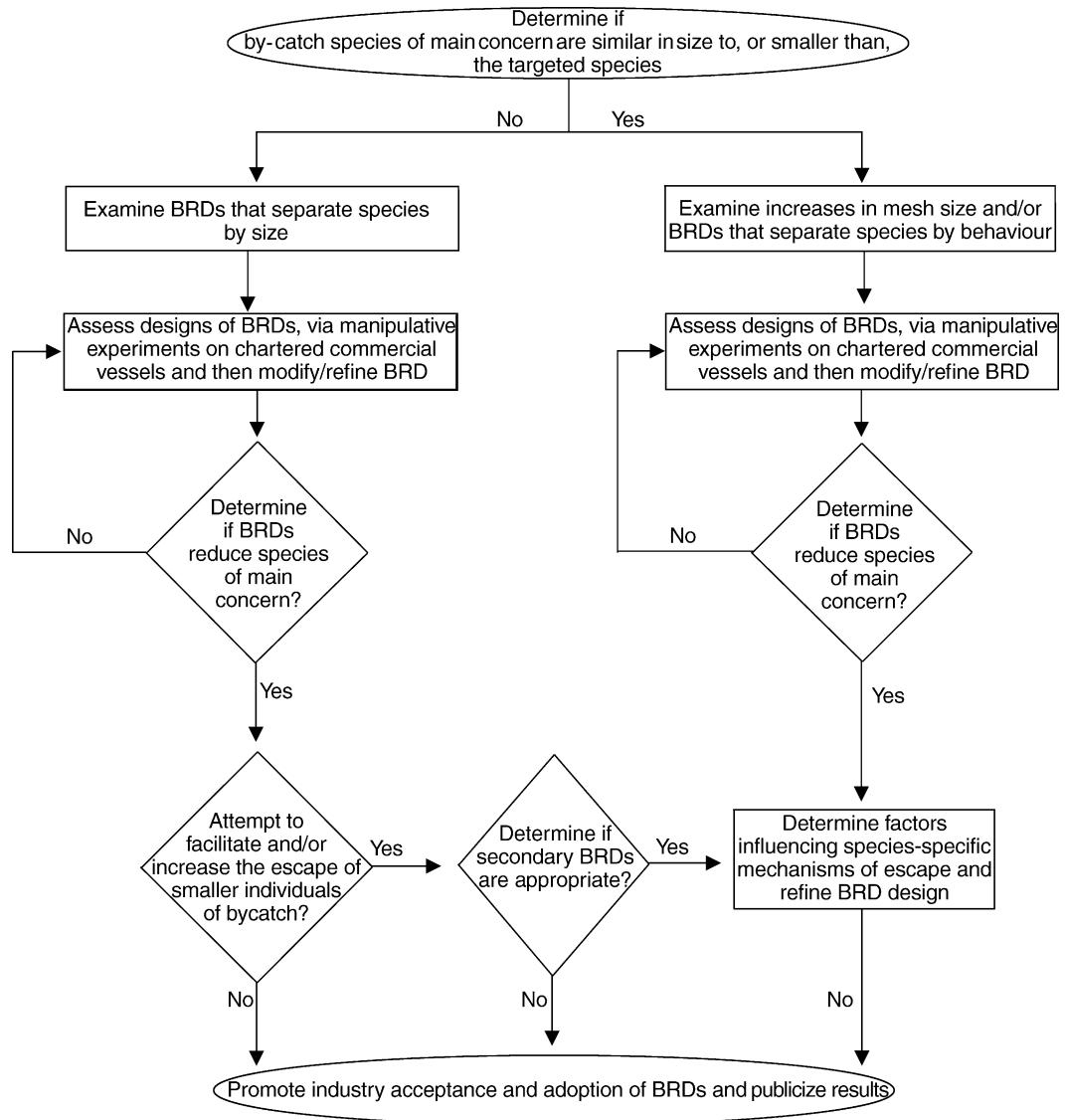
Figure 8 Summary of the logic used for developing and testing modifications in shrimp-trawl fisheries.
