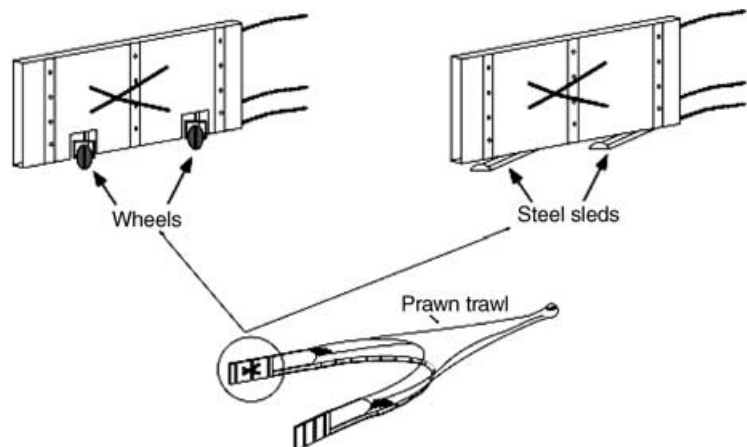
Figure 9 Two options that may reduce the ecological impacts of otter boards – using wheels and angled sleds on the base of boards.
